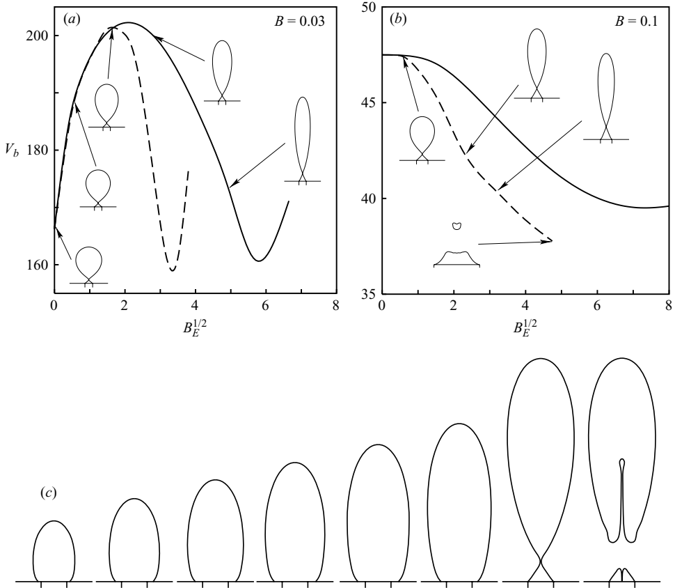
FIGURE 2. Dimensionless volume of the bubbles at detachment (scaled with a^3 ) as a function of the dimensionless electric field B^{1/2} for \epsilon = 2 (solid line) and \epsilon = 10 (dashed line), at very small values of We . (a) B = 0.03 , (b) B = 0.1 . The shapes of the bubbles immediately before detachment are shown for \epsilon = 2 in (a) and \epsilon = 10 in (b) at different values of B_E^{1/2} ; the two small vertical lines in each bubble picture denote the edge of the orifice. (c) The shapes of a bubble growing quasi-statically for B = 0.03 , B_E^{1/2} = 1.58 , \epsilon = 10 , \theta = 45^\circ , and seven equispaced values of the bubble volume. The rightmost image is not part of the quasi-static evolution. It depicts a rising bubble immediately after detachment and the new bubble left at the orifice, with re-entrant jets in both bubbles.
